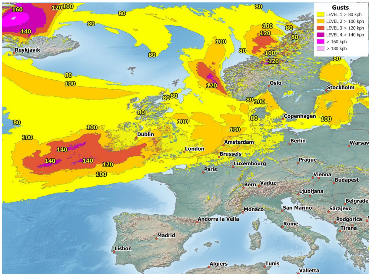
Maximum gusts in kph 10/11 March 2021. (INIT: 09 March 2021, 00 UTC. ICON-EU). Image: B. Mühr
