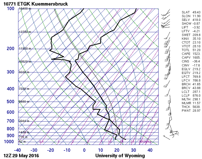
Abbildung 3: Radiosondenaufstieg Kümmerbruck (BY), 29.5.2016, 12 UTC. Quelle: Department of Atmospheric Science, University of Wyoming. http://weather.uwyo.edu/upperair/sounding.html
